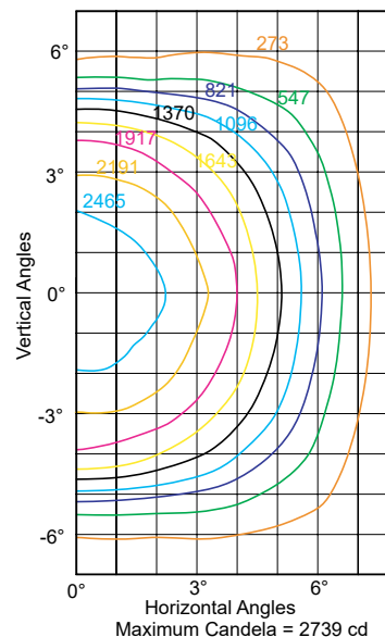
Isocandela Curves
