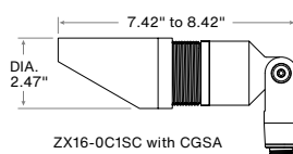
ZX16-0C1SC with CGSA
