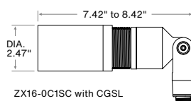
ZX16-0C1SC with CGSL
