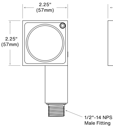
ZX16-0S1SA
