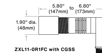
ZXL11-OR1FC with CGSS
