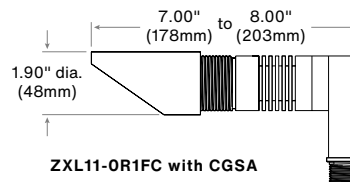
ZXL11-OR1FC with CGSA
