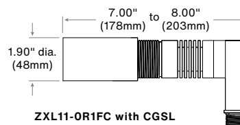
ZXL11-OR1FC with CGSL
