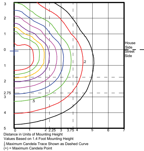
Isocandela Lines of Horizontal Illuminosity
