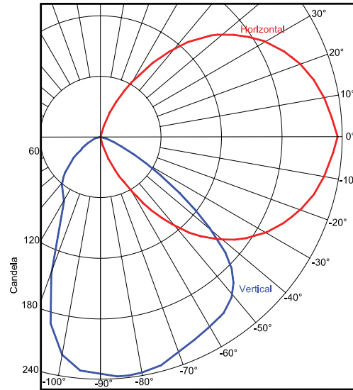
Polar Graph - Intensity
