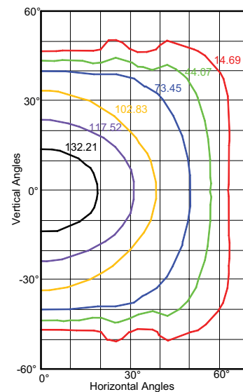
Isocandela Curves
