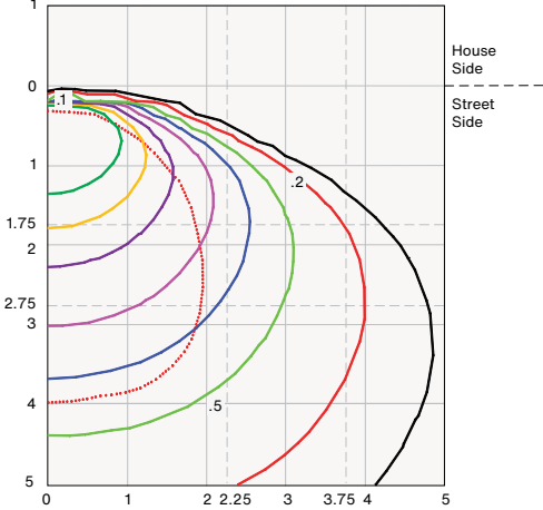
Isocandela Lines of Horizontal Illuminance
